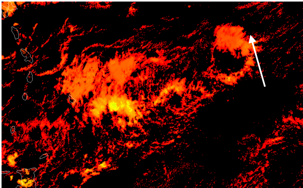
Convection at 12:35 UTC Same imagery, similar positions indicated by arrow
