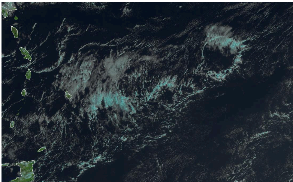
Visible imagery at 12:35 Here the blow off is evident on the north and a wonderful cold pool circle, with secondary convection and secondary cold pools on the southern edge of the ring.
