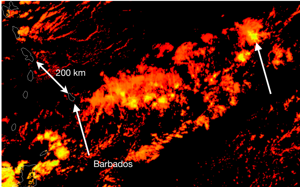
Convection at 5:45 UTC Cloud top height, green shade 5 km
